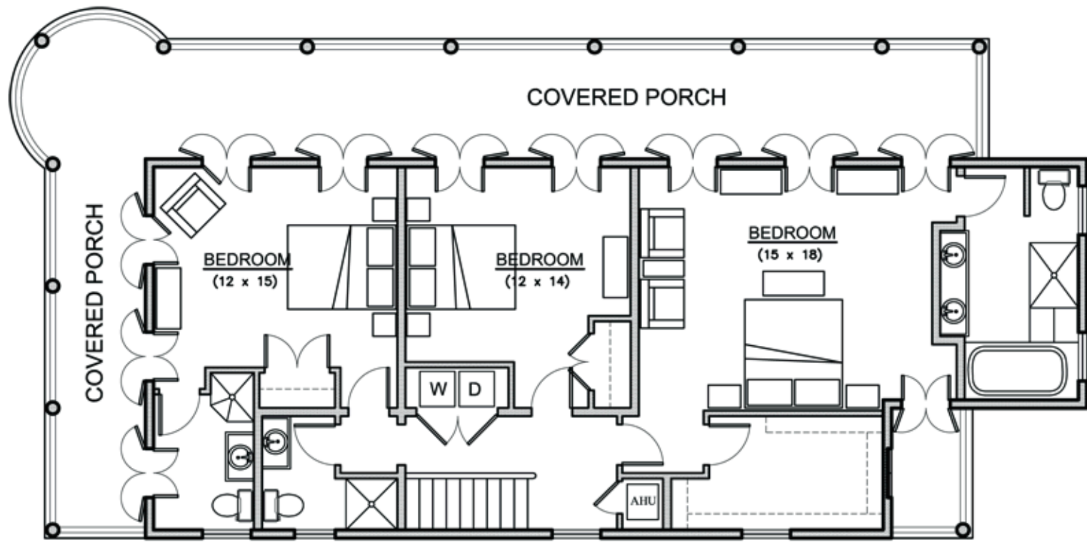
2 LEVEL TWO PLAN A2.1 SCALE: 1/4" = 1'-0"
